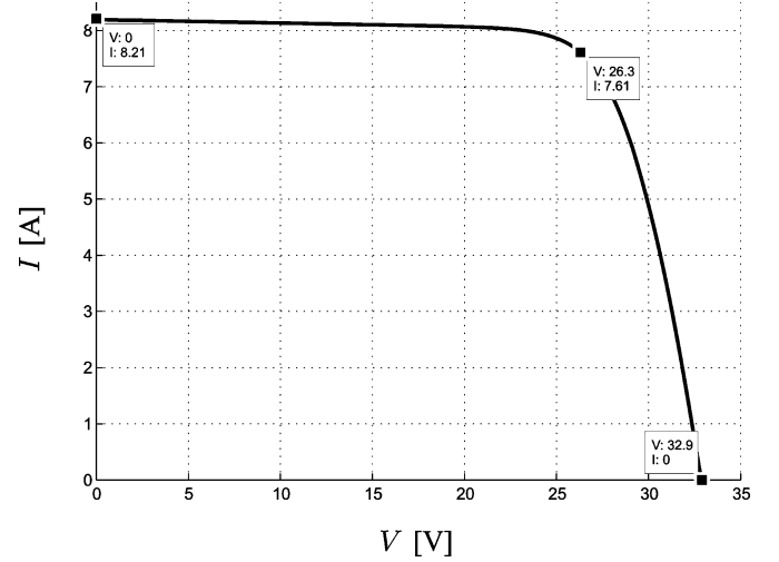
Fig. 11. I - V curve adjusted to three remarkable points.
