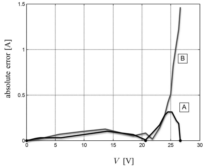
Fig. 19. Absolute errors of the model proposed in this paper (curve A) and in [23] (curve B) for the Kyocera KC200GT solar array at 75^\circ\text{C} , 1000 \text{ W/m}^2 .
